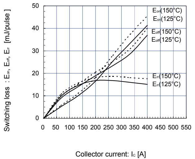
[ Inverter ]
