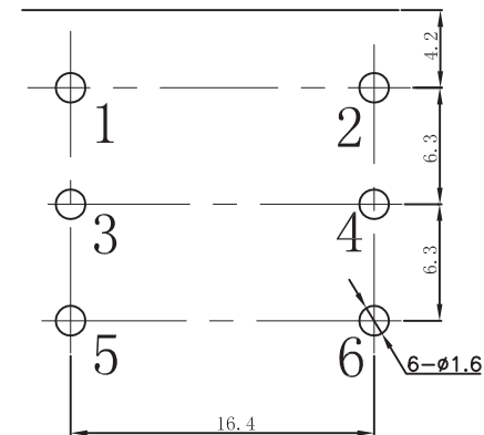
RECOMMENDED PCB LAYOUT (TOP VIEW) Tolerance: \pm 0.05
