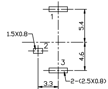
P.C.B LAYOUT VIEW
