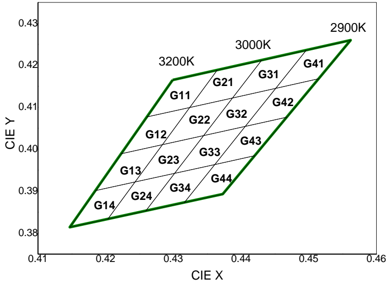
CIE Chromaticity Diagram (Warm white), T_a=25^\circ\text{C} , I_F=100\text{mA}
