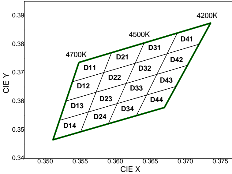
CIE Chromaticity Diagram (Neutral white), T_a=25^\circ\text{C} , I_f=100\text{mA}
