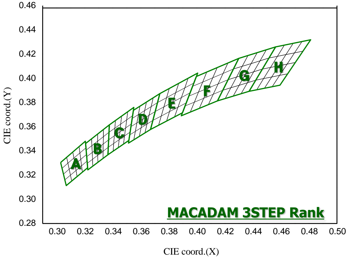
Fig 10. CIE Chromaticity Diagram, T_a=25^\circ\text{C} , I_f=100\text{mA}
