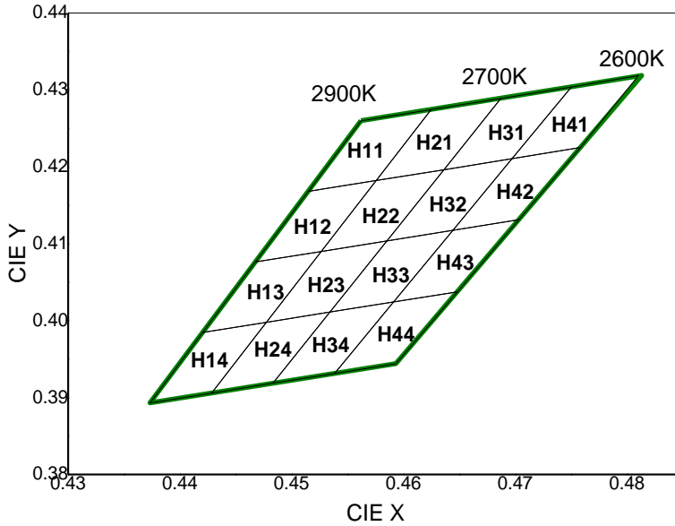
CIE Chromaticity Diagram (Warm white), T_a=25^\circ\text{C} , I_F=100\text{mA}
