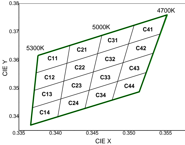
CIE Chromaticity Diagram (Cool white), T_a=25^\circ\text{C} , I_f=100\text{mA}
