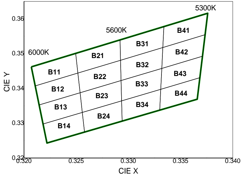
CIE Chromaticity Diagram (Cool white), T_a=25^\circ\text{C} , I_f=100\text{mA}
