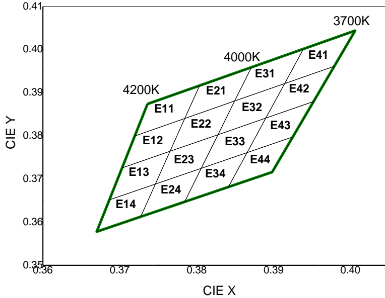
CIE Chromaticity Diagram (Neutral white), T_a=25^\circ\text{C} , I_f=100\text{mA}
