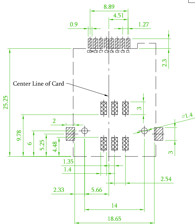
Recommended PCB Layout (PCB TOLERANCE \pm 0.05 )
