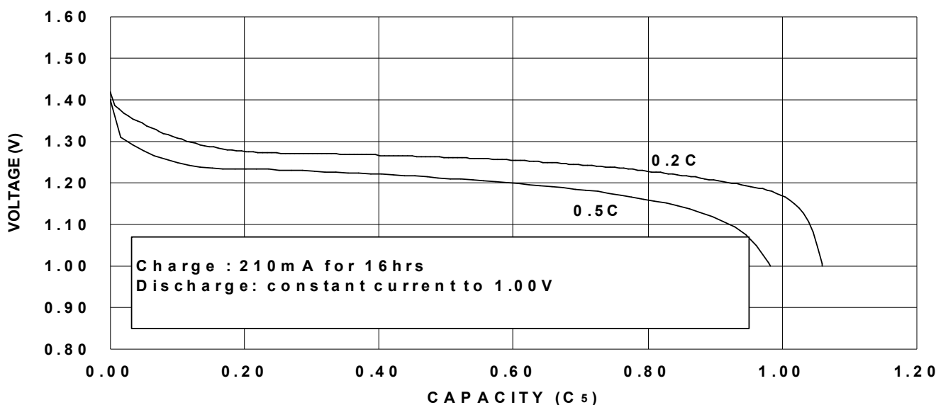
DISCHARGE CHARACTERISTICS OF BPI-49AA2100mAh CELL
