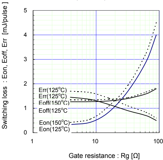
[ Inverter ]
