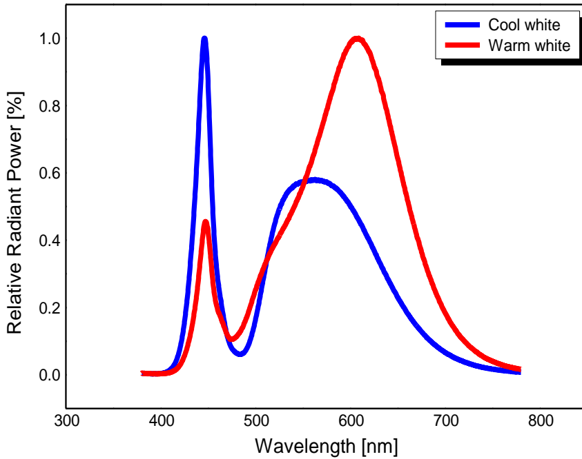
Fig 1. Color Spectrum, T_a = 25^\circ\text{C} , I_F = 180\text{mA} , \text{RH}30\%
