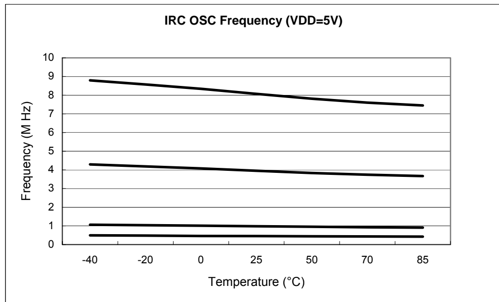
Fig 8-2 Internal RC OSC Frequency vs. Temperature, VDD=5V
