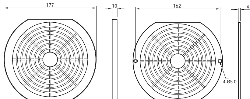
PF 17 For 172mm Fan
