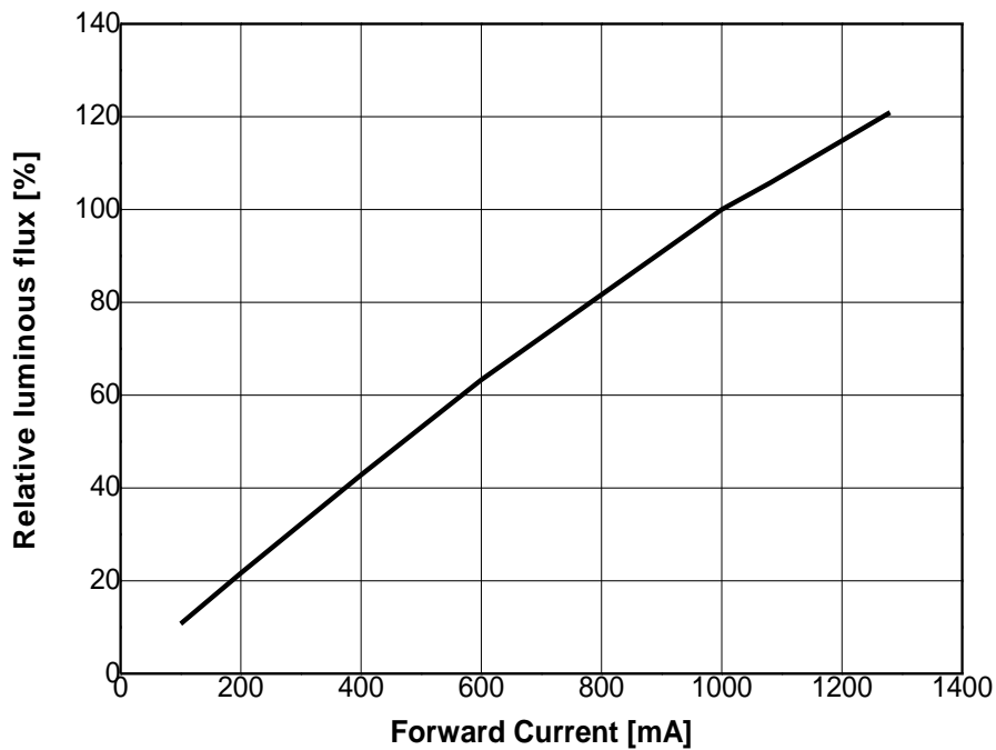
Fig 4. Forward Current vs. Relative Luminous Flux, Ta=25 °C
