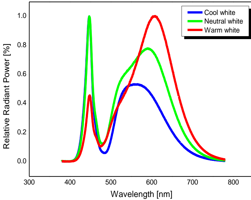
Fig 1. Color Spectrum, Ta = 25°C, IF = 1000mA, RH30%
