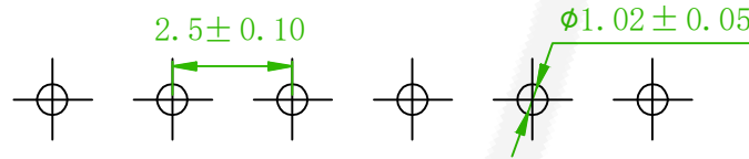
Recommended PCB Layout (PCB TOLERANCE ±0.05)
