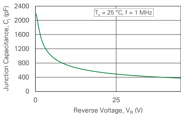
Figure 3. Typical Junction Capacitance vs. Reverse Voltage
