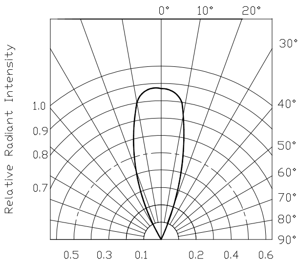
RADIATION DIAGRAM
