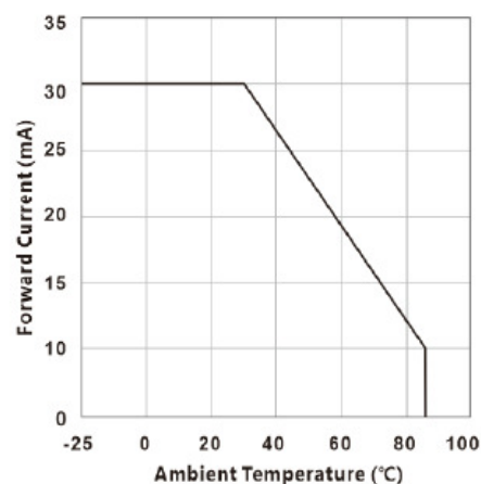
Forward Current V.S. Derating Curve
