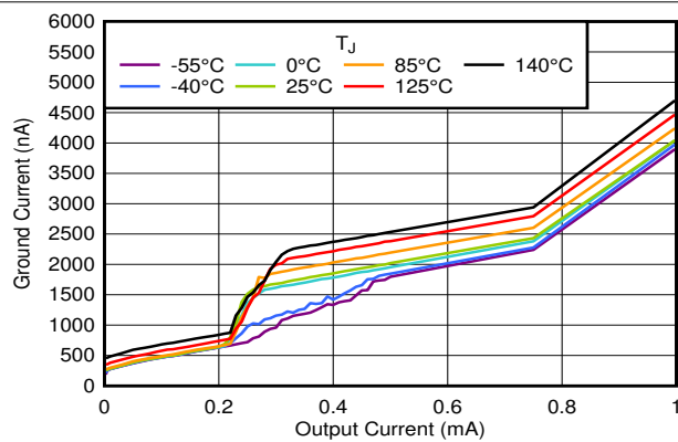
Figure 6-5. I_Q vs I_{OUT} and Temperature Up to 1 mA
