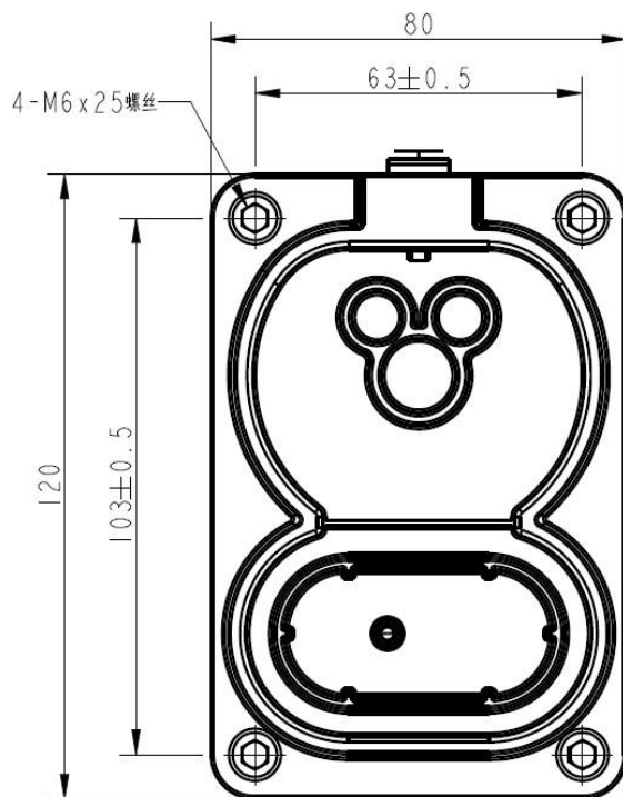
Exterior size reference
