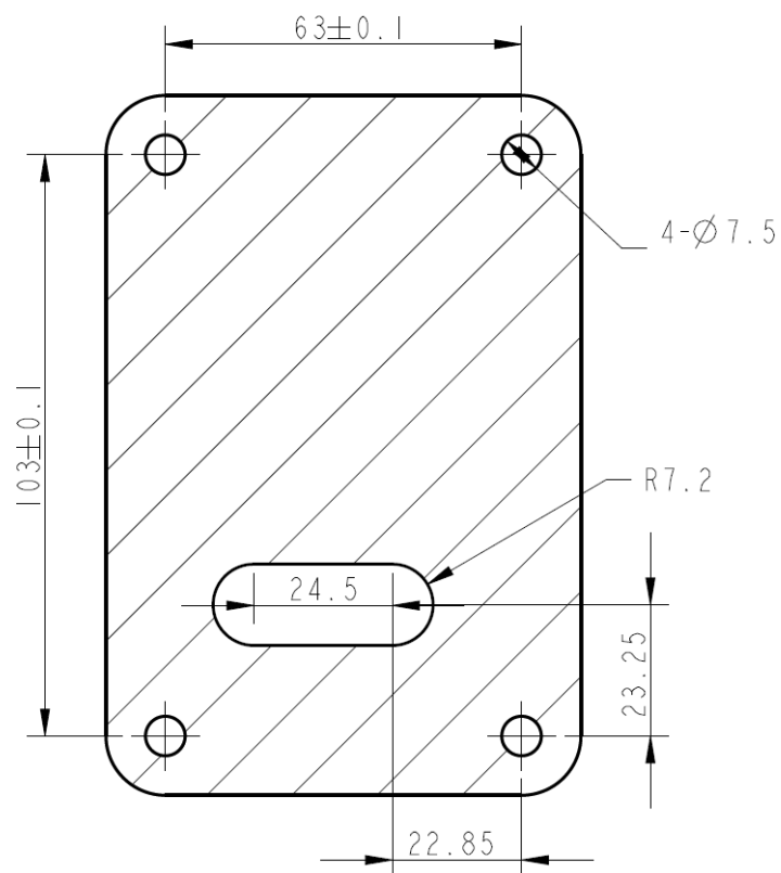
Mounting panel cutout size reference (screw torque 6 \pm 0.2 \text{N} \cdot \text{m} )
