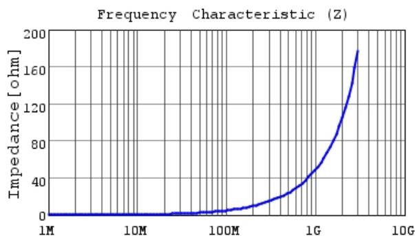
LQW15AN8N0G80 |Z|
