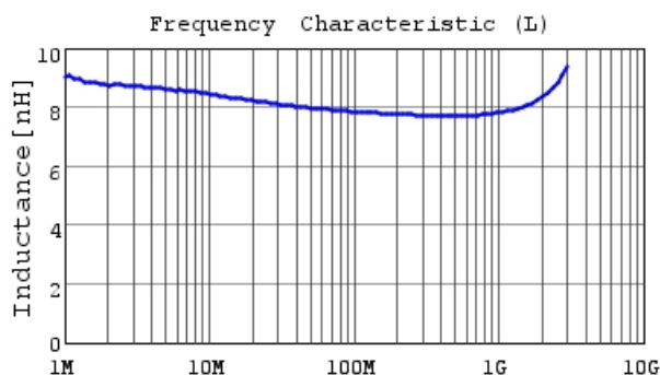
LQW15AN8N0G80 L
