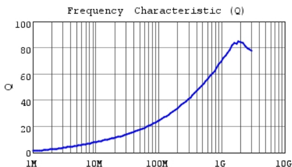
LQW15AN8N0G80 Q
