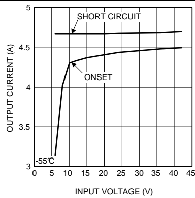
Figure 27. Current Limit 3.3 V OUT at -55°C
