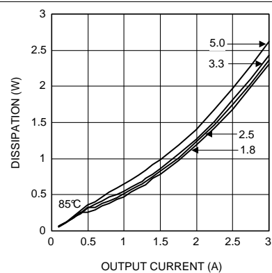
Figure 14. Dissipation 12-V Input at 85°C
