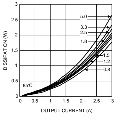
Figure 10. Dissipation 6-V Input at 85°C
