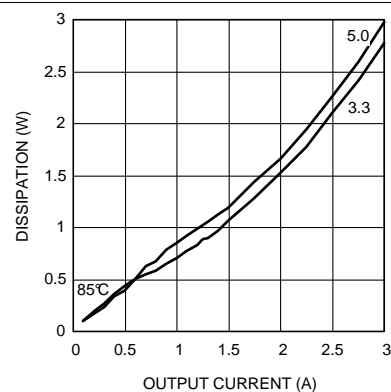
Figure 16. Dissipation 24-V Input at 85°C
