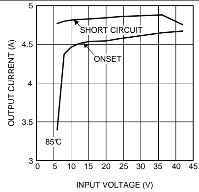
Figure 26. Current Limit 3.3 V OUT at 85°C
