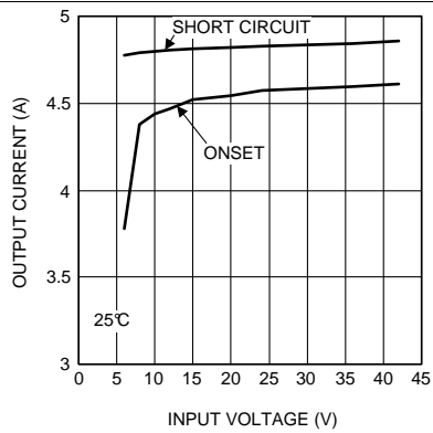
Figure 25. Current Limit 3.3 V OUT at 25°C
