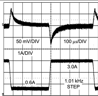
Figure 21. Line and Load Regulation at -55°C
