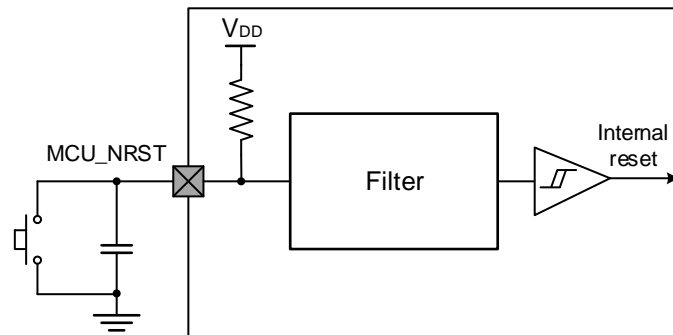
NRST pin protection recommended circuit design
