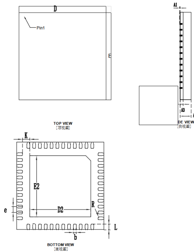
Figure 7-2. QFN48 6x6 package
