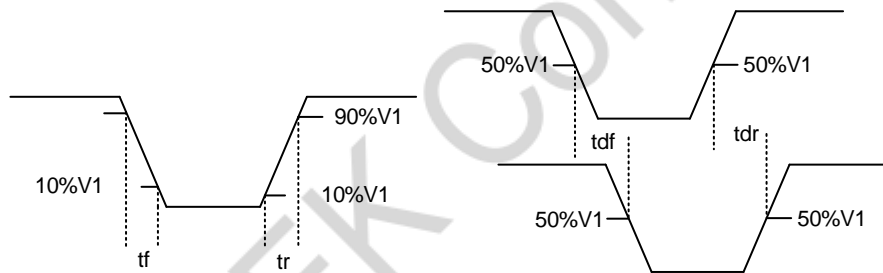
I/O AC characteristic definition
