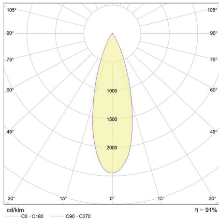
CREE XPG3
