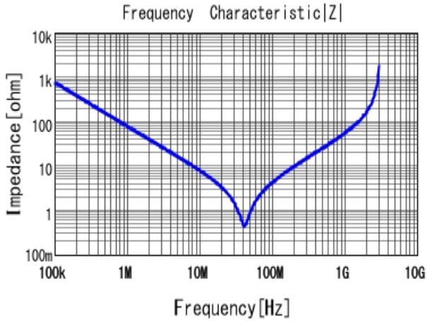
■ DE2E3KY222MN2AM01F |Z| DCOV, 20degC
