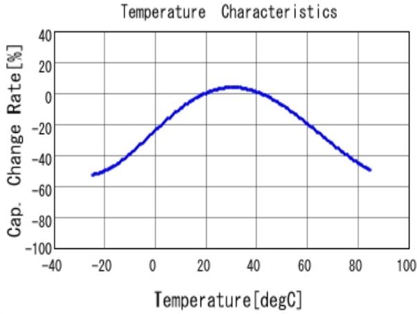
■ DE2E3KY222MN2AM01F C-Temp. capchange, DCOV, AC1Vrms
