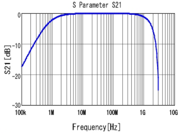
■ DE2E3KY222MN2AM01F S21 DCOV, 20degC
