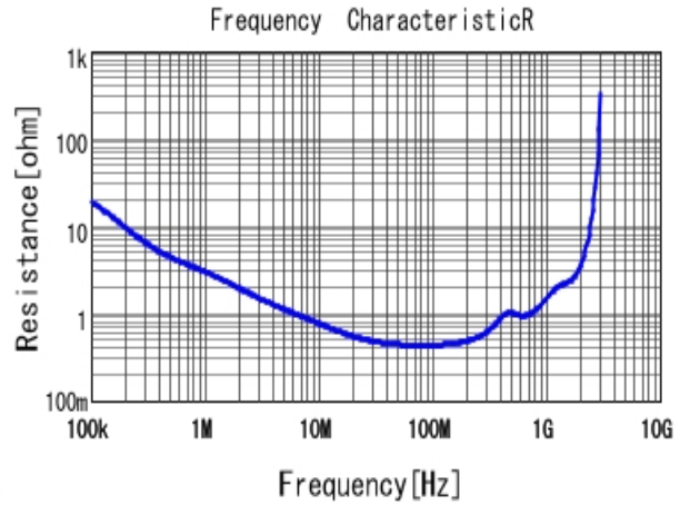
■ DE2E3KY222MN2AM01F R DCOV, 20degC
