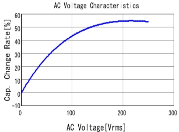
■ DE2E3KY222MN2AM01F C-AC Voltage capchange, DCOV, 20.0
