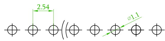
Recommended PCB Layout (PCB TOLERANCE ±0.1)
