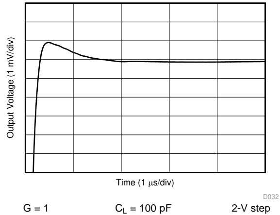
Figure 26. Large-Signal Settling Time (Positive)
