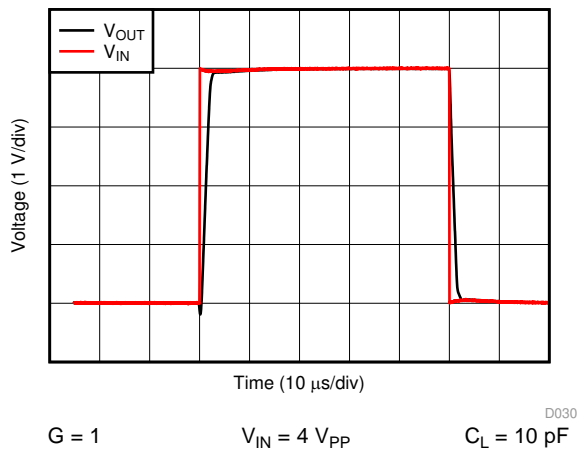
Figure 24. Large-Signal Step Response
