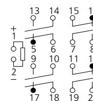
Schematic ( BOTTOM VIEW )
