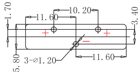
PCB Layout Diagram Top View
