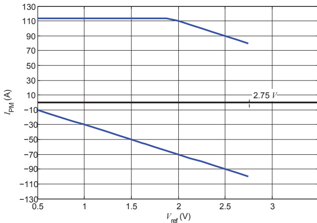
Figure 33: Measuring range versus external V_{ref} LESR 25-NP
