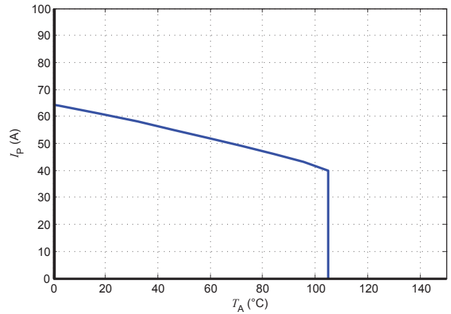
Figure 22: I p vs T A for LESR 15-NP
