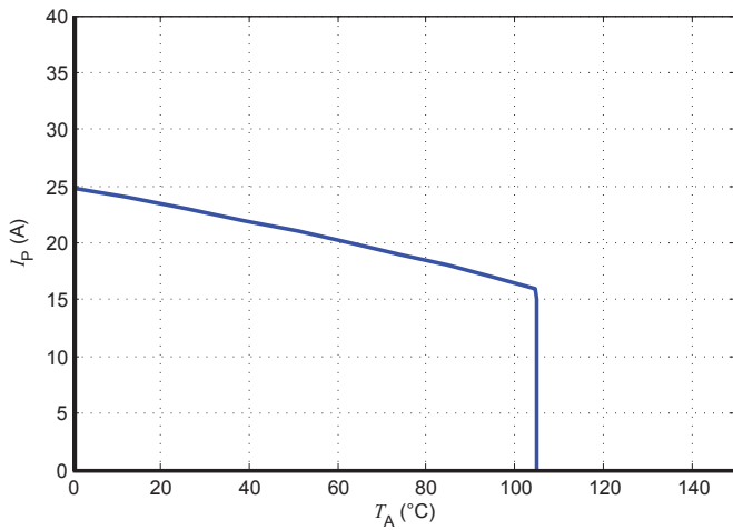
Figure 21: I p vs T A for LESR 6-NP
