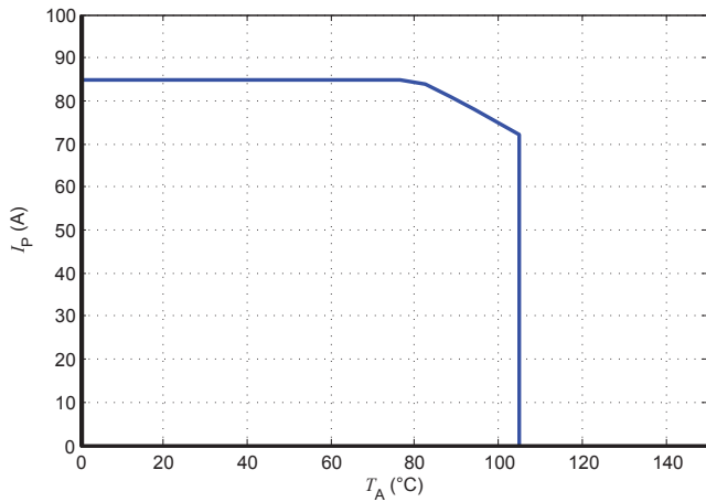
Figure 23: I p vs T A for LESR 25-NP
