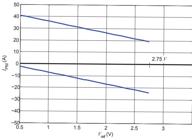
Figure 31: Measuring range versus external V_{ref} LESR 6-NP
