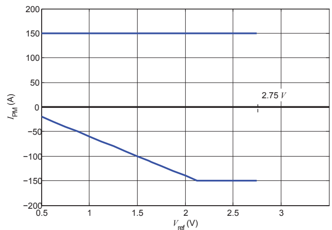
Figure 34: Measuring range versus external V_{ref} LESR 50-NP
