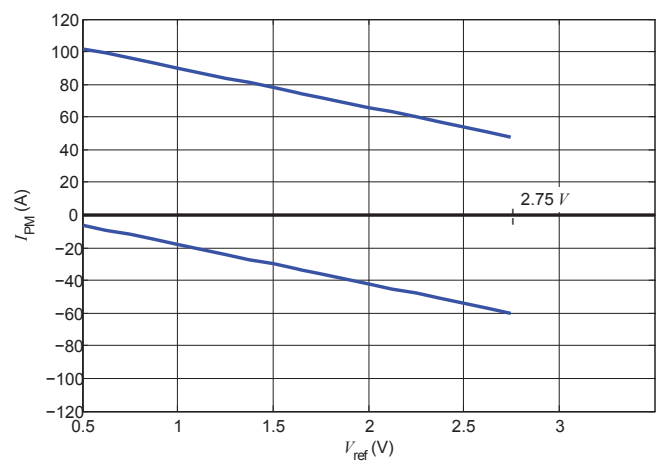
Figure 32: Measuring range versus external V_{ref} LESR 15-NP
