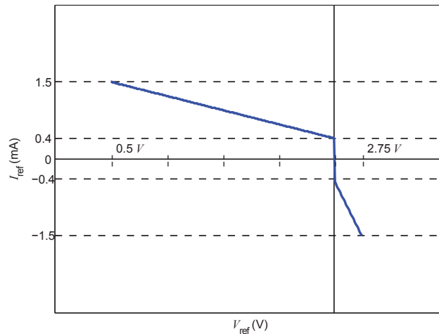
Figure 30: I_{ref} versus forced external V_{ref}
