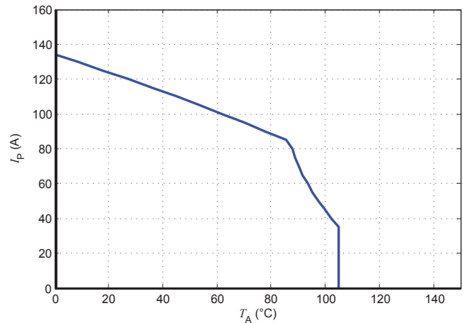
Figure 24: I p vs T A for LESR 50-NP
