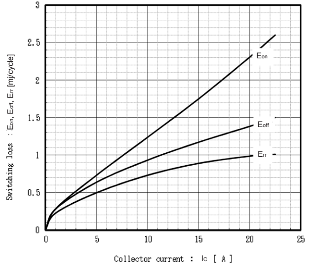
Switching Loss vs. Collector Current (typ.) V_{bc}=600V, V_{cc}=15V, T_j=125^\circ C
