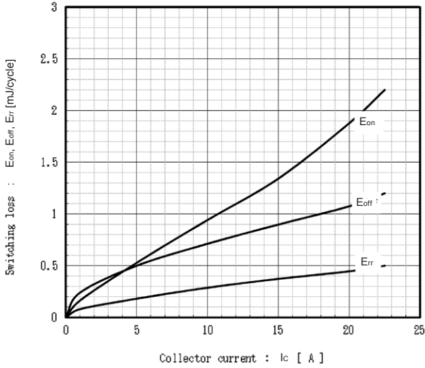
Switching Loss vs. Collector Current (typ.) V_{bc}=600V, V_{cc}=15V, T_j=25^\circ C
