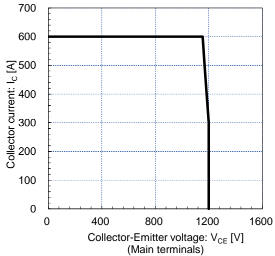
Reverse bias safe operating area (max.) +V_{GE}=15V, -V_{GE}=15V, R_g=3.3\Omega, T_j=125^\circ C
