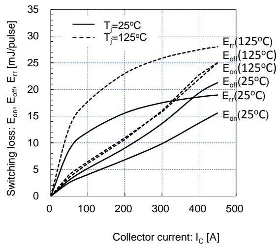
Switching loss vs. Collector current (typ.) V_{CC}=600V, V_{GE}=\pm 15V, R_g=3.3\Omega, T_j=25, 125^\circ C
