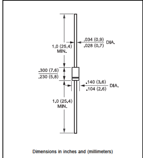
DO-15
