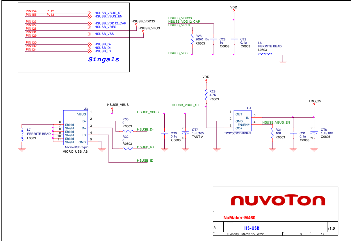
Figure 5-7 High-speed Circuit
