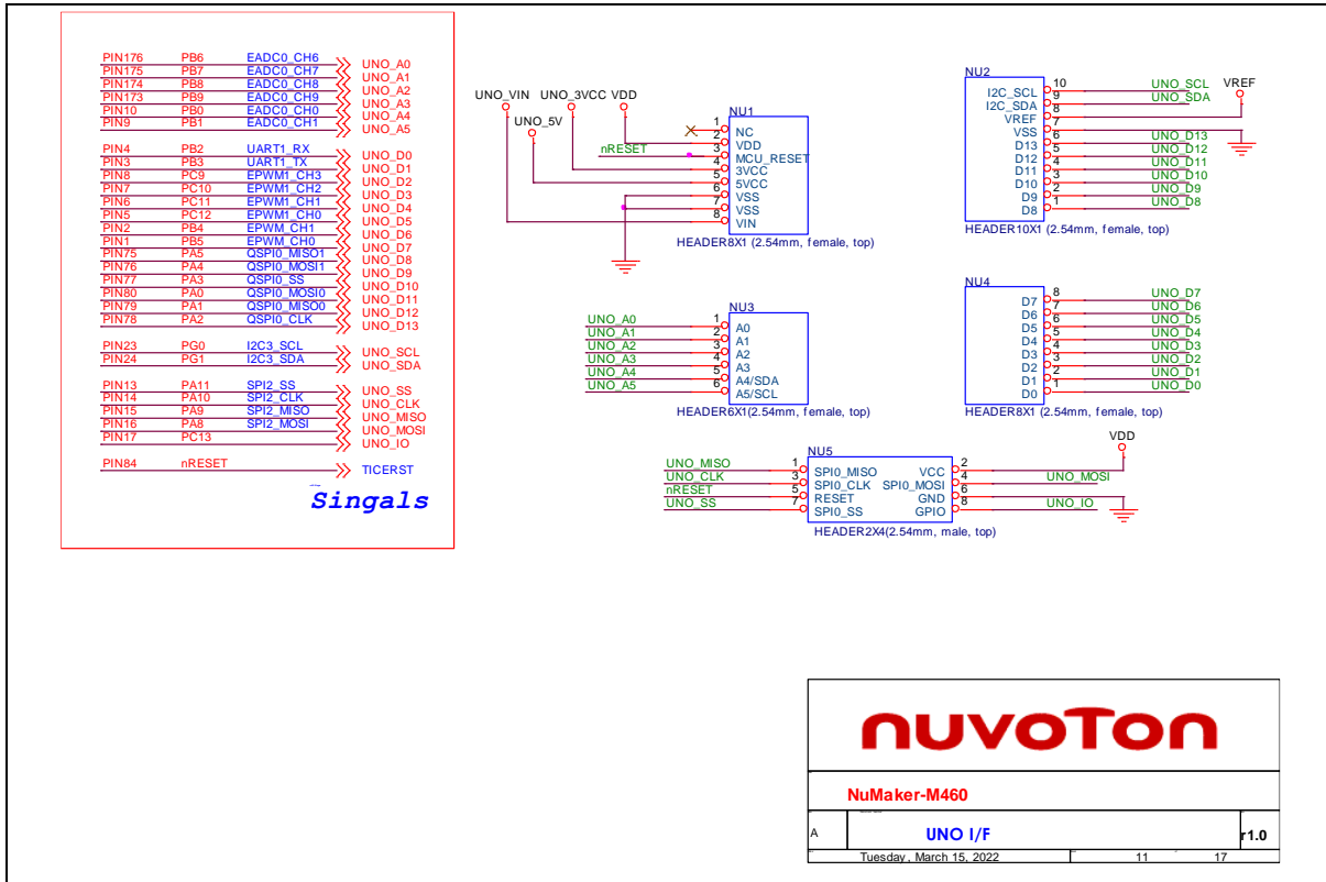
Figure 5-10 Arduino Uno I/F Circuit
