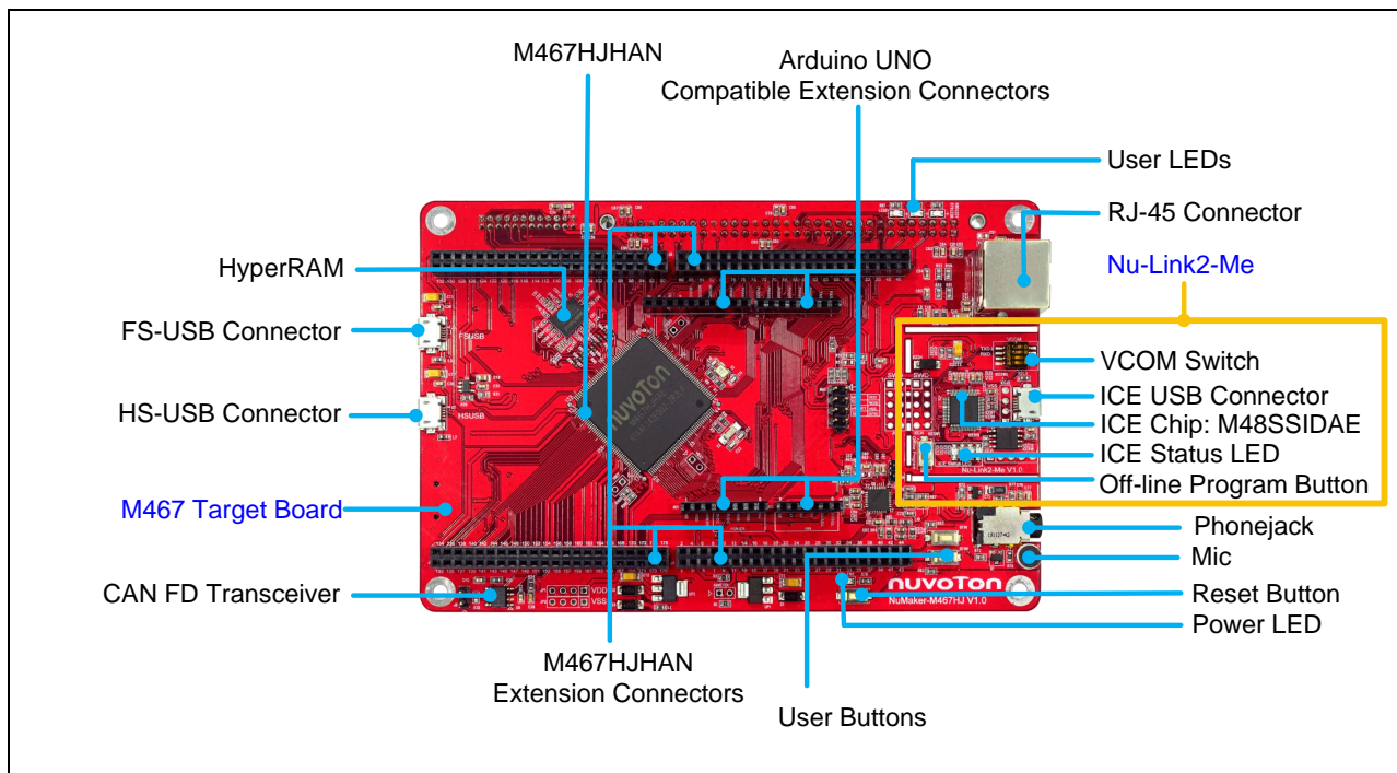
Figure 3-1 Front View of NuMaker-M467HJ
