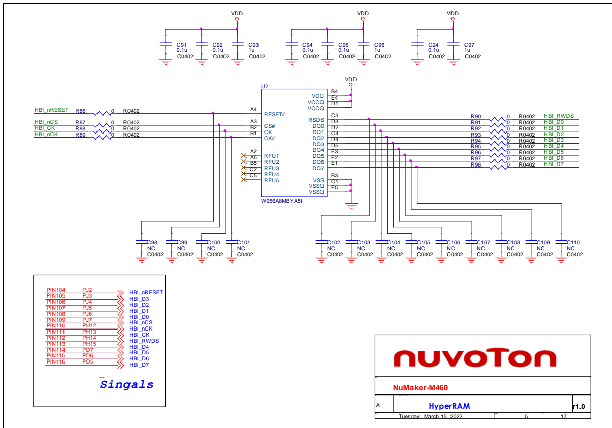
Figure 5-4 HyperRAM Circuit
