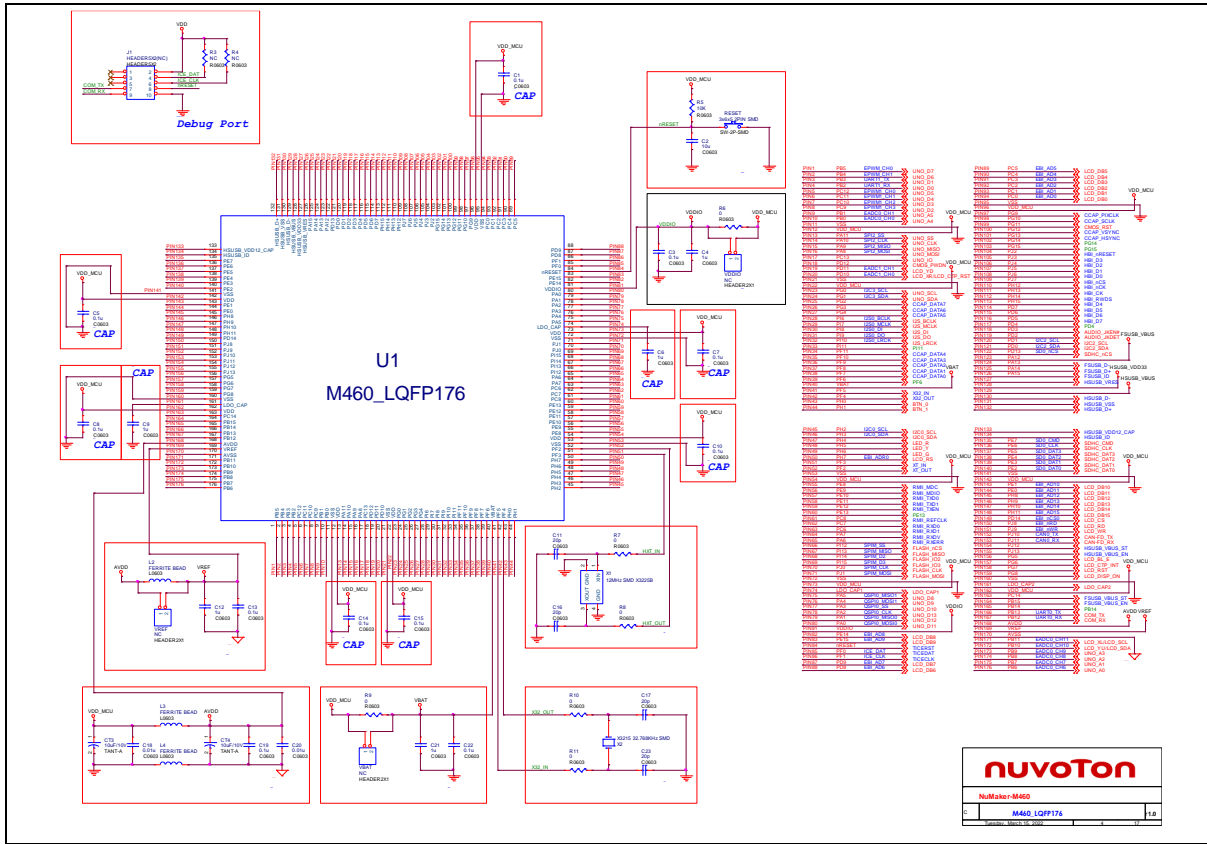
Figure 5-3 M467HJHAN Circuit
