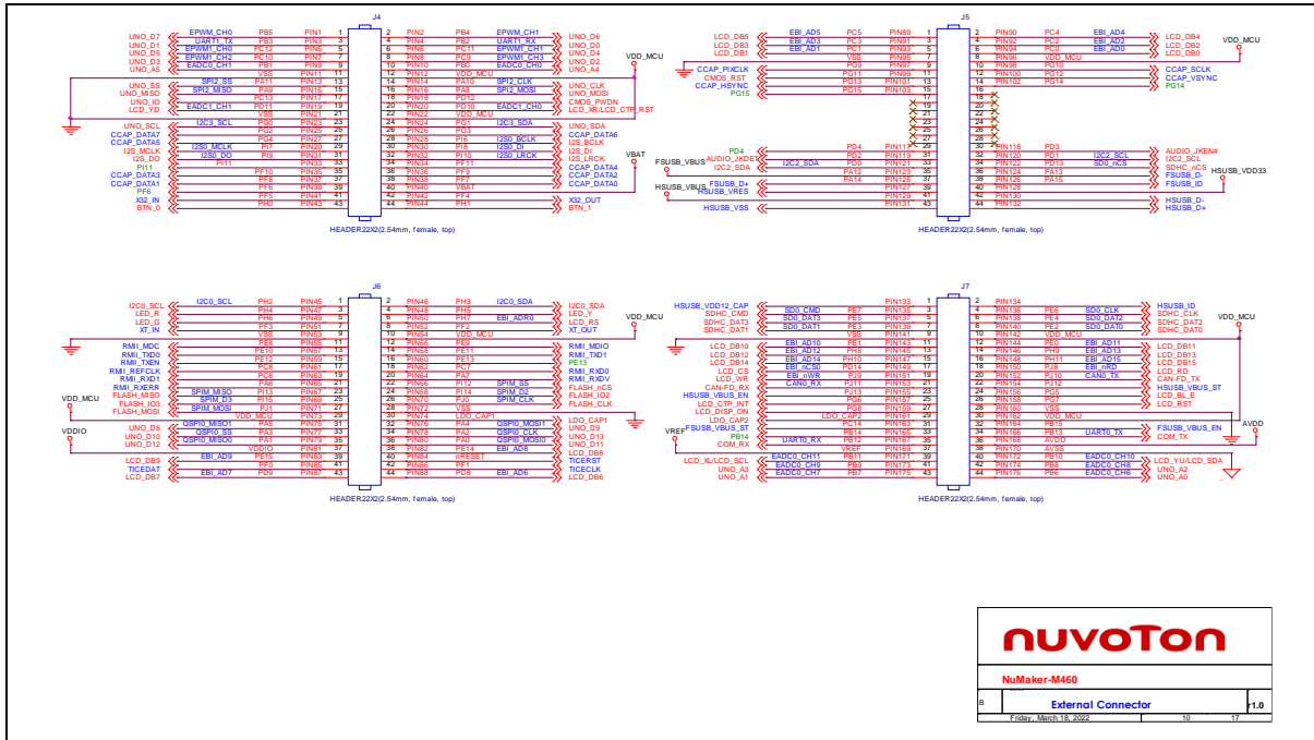
Figure 5-9 Extension Connectors Circuit
